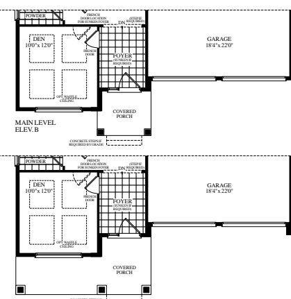
MAIN LEVEL ELEV. B
