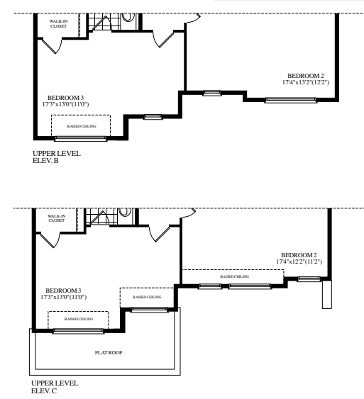
UPPER LEVEL ELEV. B
