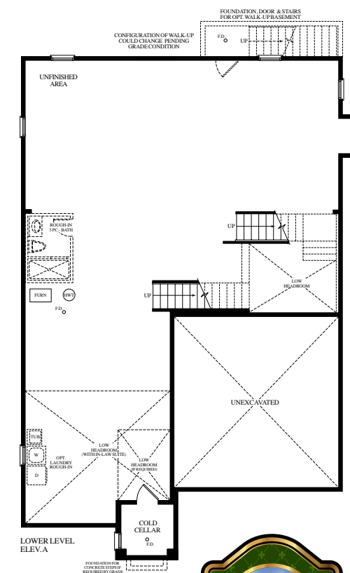
LOWER LEVEL ELEV. A
