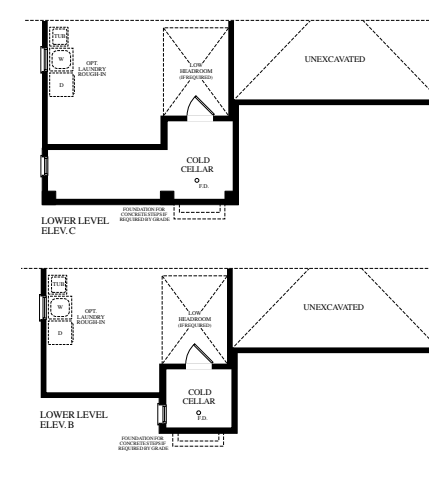
LOWER LEVEL ELEV. B
